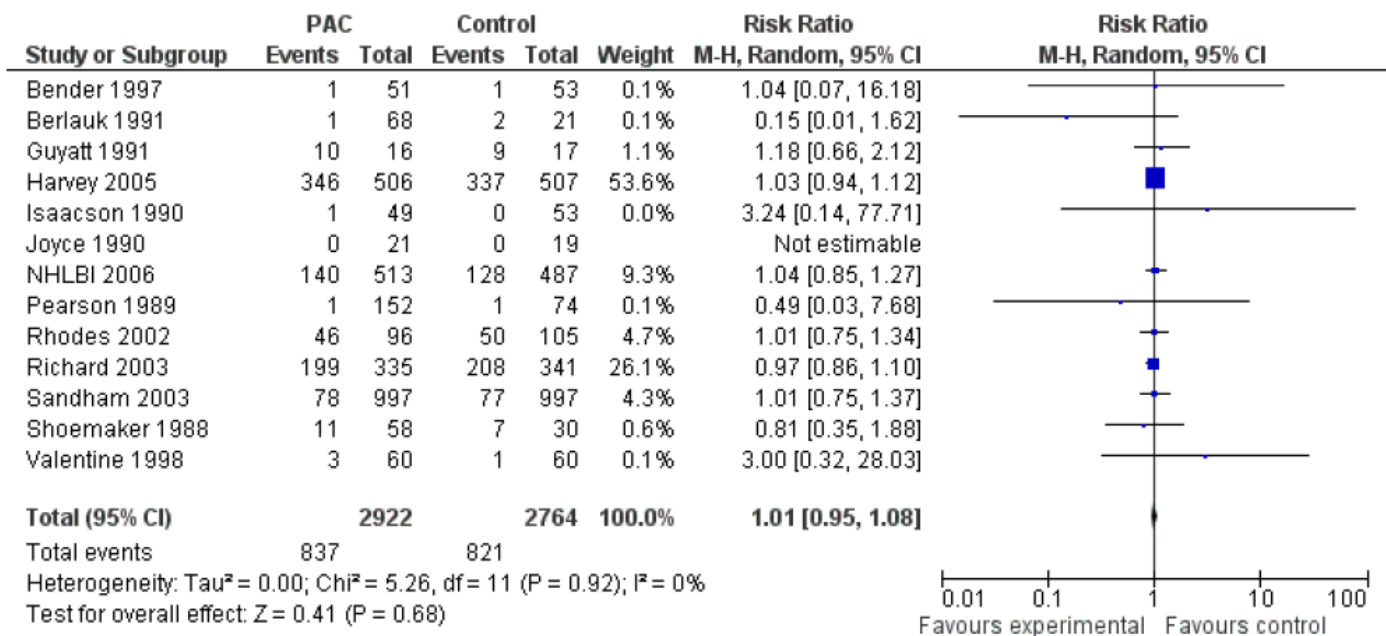
Figure 2. Forrest plot of mortality in combined medical and surgical patients for PAC vs no-PAC (Adapted from 6 ).
